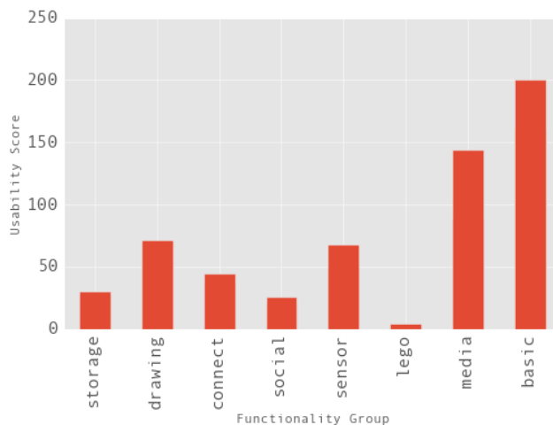
Figure 7. Usability Score (Ratio of the Number of Projects to Median Number of Unique Blocks) of Functionality Groups
