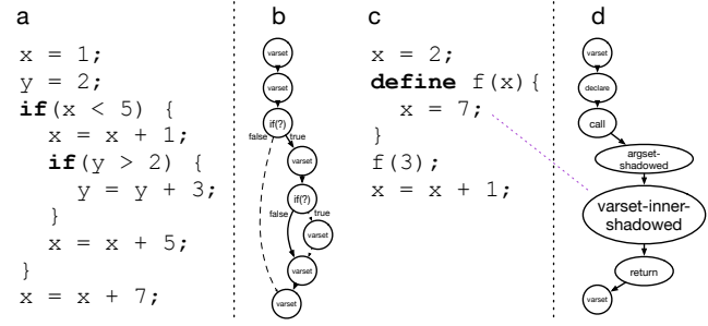
Figure 2: (a) An example item (item 28) and (b) the SemCFG path it attempts to assess. (c) A code example with (d) SemCFG with data flow varset-inner-shadowed.
